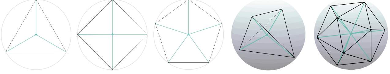
Figure 1. Frame vectors X (blue) and their convex hulls forming convex regular polytopes P_X . From left to right: Mercedes-Benz, Square, and Pentagon frame in \mathbb{R}^2 , Tetrahedron and Icosahedron frame in \mathbb{R}^3 . The unit ball \mathbb{B} is outlined in gray.
