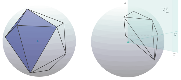
Figure 3. Non-regular polytopes. Left: The estimated bias values \alpha_i^{\mathbb{B}} are computed from the largest adjacent facet of x_i . Hence, the less regular the normalized frame elements are distributed on the sphere, the smaller \alpha^{\mathbb{B}} becomes. Right: The frame is non-negatively omnidirectional since \bigcup_{j \in J^+} F_j \supseteq \mathbb{R}_+^n , but not omnidirectional.
