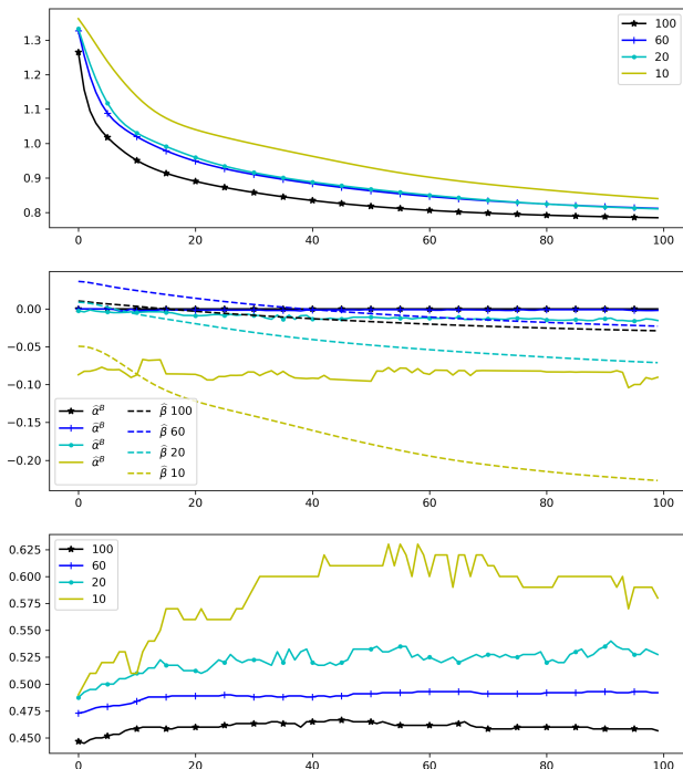
Figure 4. Averaged quantities (across 10 iterations) related to a ReLU-layer over 100 epochs of training with different redundancies m = |I| . Top: Cross entropy loss on the validation set. Mid: Mean of the trained biases, \hat{\beta} (dashed), and mean of the estimated upper biases on \mathbb{B}_r , \hat{\alpha}^{\mathbb{B}} (solid). Bottom: Proportion of learned bias values that are smaller than the estimations, i.e. \#(\beta_i \leq \alpha_i^{\mathbb{B}})/m , indicating the injectivity trend.
