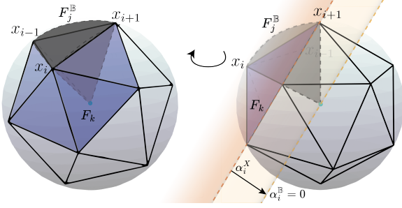
Figure 2. Geometrical intuition of the PBE for the Icosahedron frame on \mathbb{B} . Consider x_i . Left: The (blue) filled facets are used to compute \alpha_i^{\mathbb{B}} . The (gray) darker piece (dashed border) indicates F_j^{\mathbb{B}} . Right: Rotated perspective of the left image. The affine half-space \Omega_i = \{x \in \mathbb{R}^n : \langle x, x_i \rangle \geq \alpha_i^X, i \in I_{F_j}\} , indicated by the left-most area with decreasing opacity (orange) contains all vectors such that all vertices of the adjacent facets are active. Since \alpha_i^X \geq 0 , the brighter (yellow) half-space represents the solution \alpha_i^{\mathbb{B}} = 0 .
